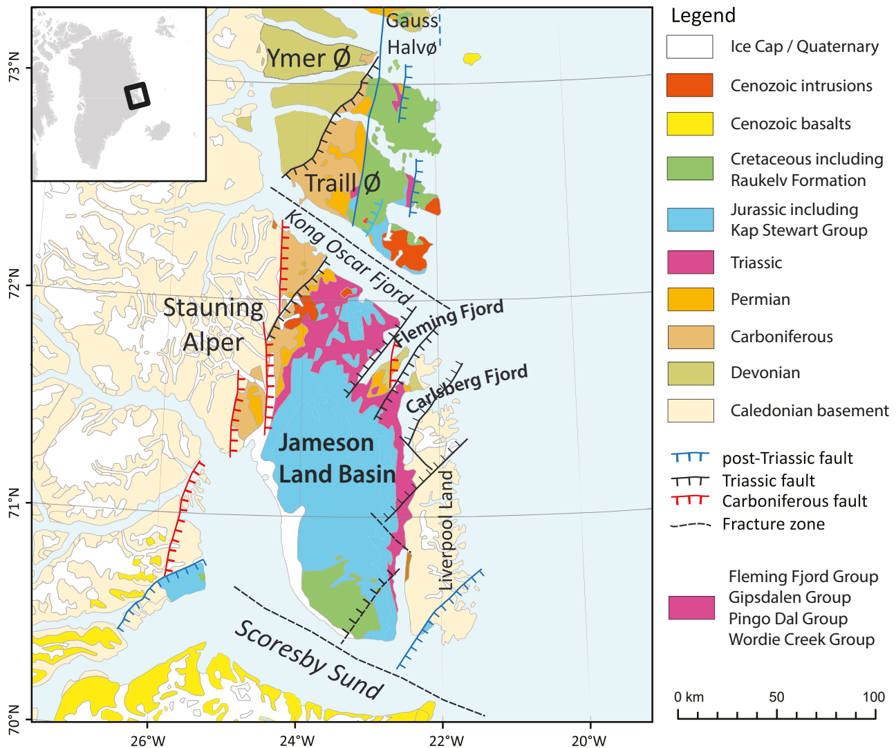
Fig. 1. Geological map of central east Greenland with the Jameson Land Basin. The basin is bounded by the N-S stretching Liverpool Land to the east and the Stauning Alper to the west. To the north and south, the basin is demarcated by fracture zones in the Kong Oscars Fjord and the Scoresby Sund respectively. Other Triassic faults are also indicated. Geological map modified from Guarnieri et al. 2017.
