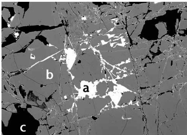
Fig. 25. Fractures in fresh eudialyte (b) filled with mineral Uk2 (a). Black areas (c) are either a silicate mineral (K-feldspar or analcime) or epoxy-filled cavities. Sample 151428, circular pegmatite. Width of image 0.61 mm.
