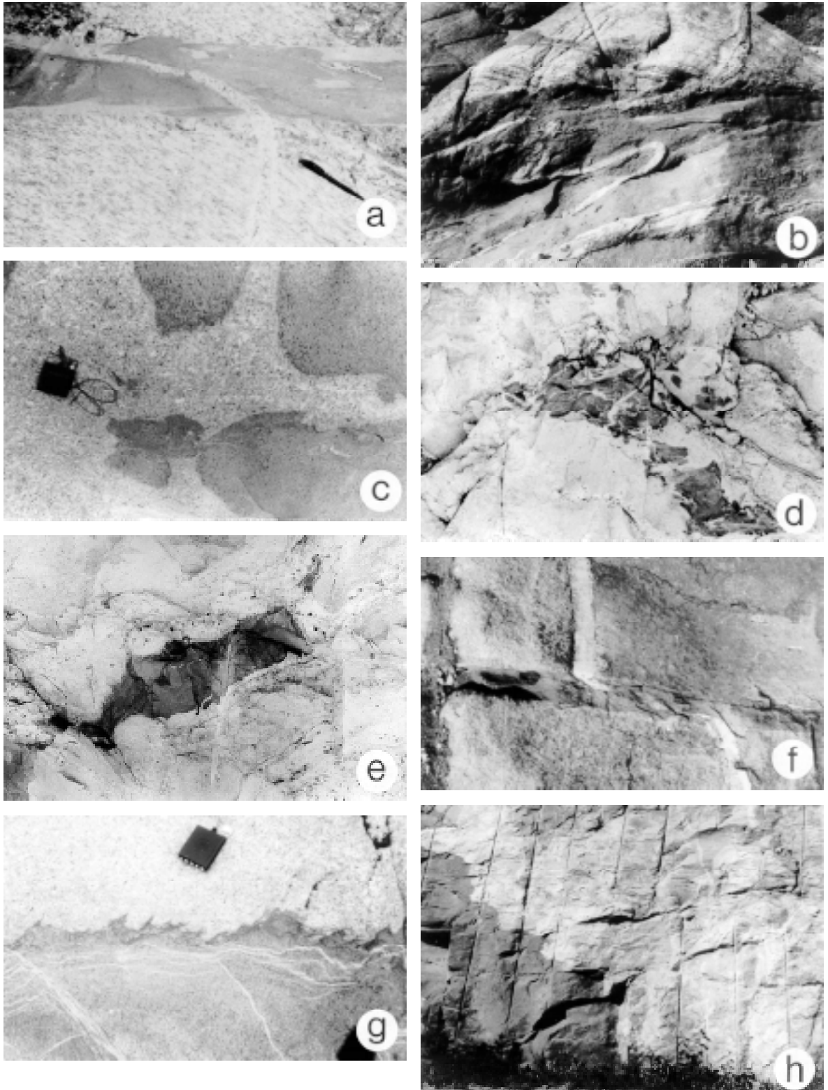
Fig. 4. Examples of shapes, margins and internal structures of monzonite dykes and other minor monzonite bodies (dark on the photographs). b is from loc. 3, h from loc. 2. See text for further explanations. Approximate heights of photos: a: 75 cm, b: 1.5 m, c: 60 cm, d: 75 cm, e: 60 cm, f: 75 cm, g: 50 cm, h: 4 m.
