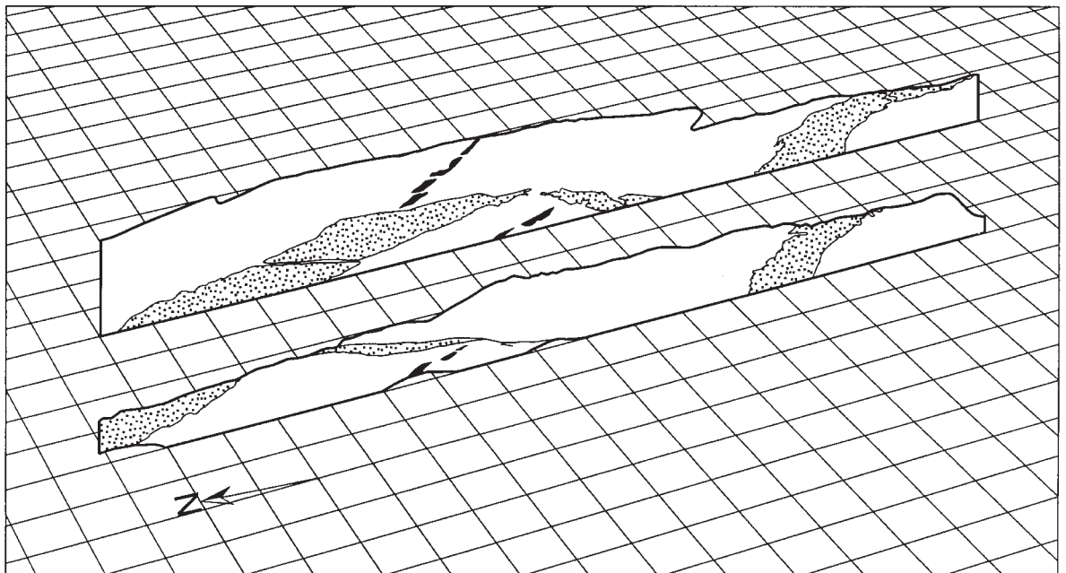
Fig. 7. Above: Road cuts at locality 2, no vertical exaggeration. Below: set piece diagram showing relative position of the road cuts. Side length of squares is 2m.
