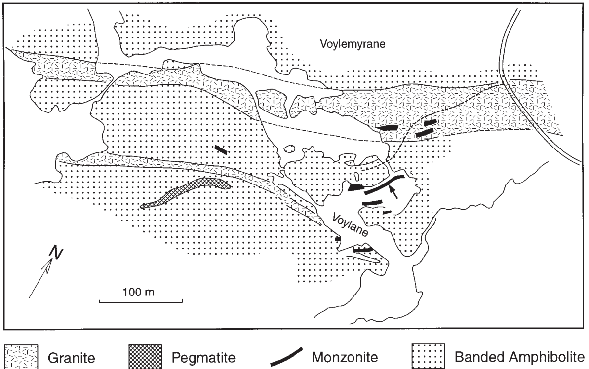
Fig. 8. Geological map of the area around Voylane (loc. 3). Stippled heavy line is a foot path from the gravel road in the upper right corner towards the locality. Arrow points to the monzonite dyke that was subjected to detailed structural investigations. The dyke is only visible at low water levels in Voylane.
