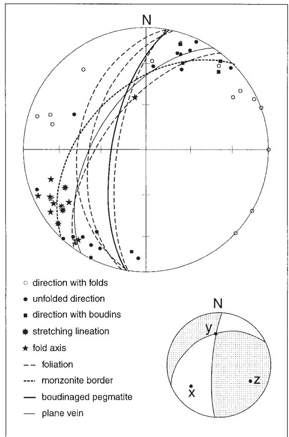
Fig. 12. Above: equal are projection of structural elements measured at locality 3. Below: shortening fields (stippled) and extension fields.
