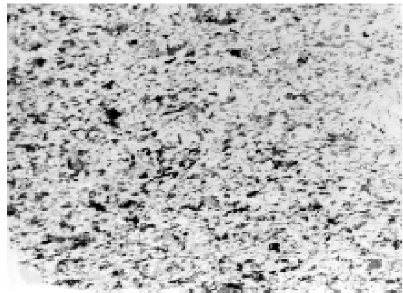
Fig. 6. Above: strongly foliated and lineated monzonite dyke with folded granitic sheets, the lineation is almost parallel to the surface of the outcrop, locality 3, ball pen as scale. Right: thin section showing foliation in a monzonite dyke (plane light), the monzonite also contains a lineation which is perpendicular to the section. Horizontal length of photo is 2 cm.
