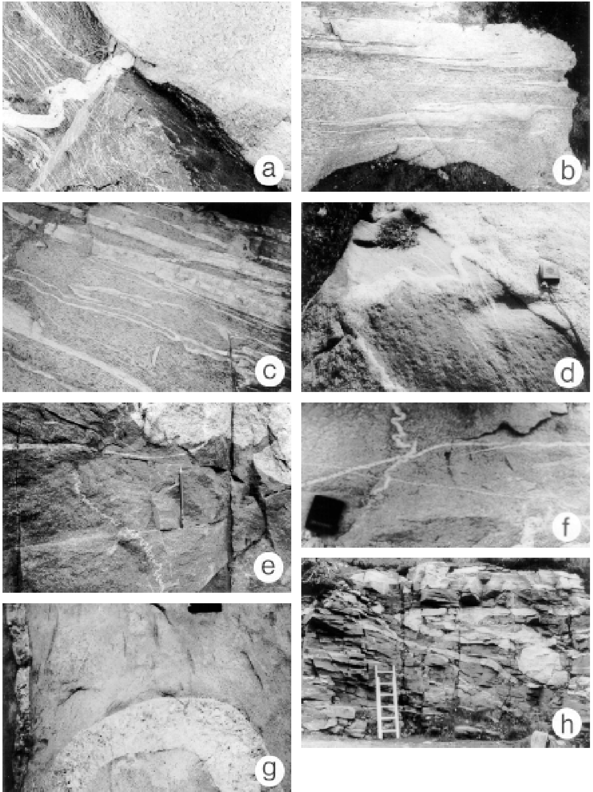
Fig. 5. Examples of shapes, margins and internal structures of monzonite dykes and other minor monzonite bodies (dark on the photographs). a, b and c are from loc. 3, e and f are from loc. 2, h show part of the outcrop at loc. 1 with structures cut at a low angle to the foldaxes. See text for further explanations. Approximate heights of photos: a: 75 cm, b: 60 cm, c: 60 cm, d: 80 cm, e: 50 cm, f: 40 cm, g: 35 cm, h: 4.5 m.
