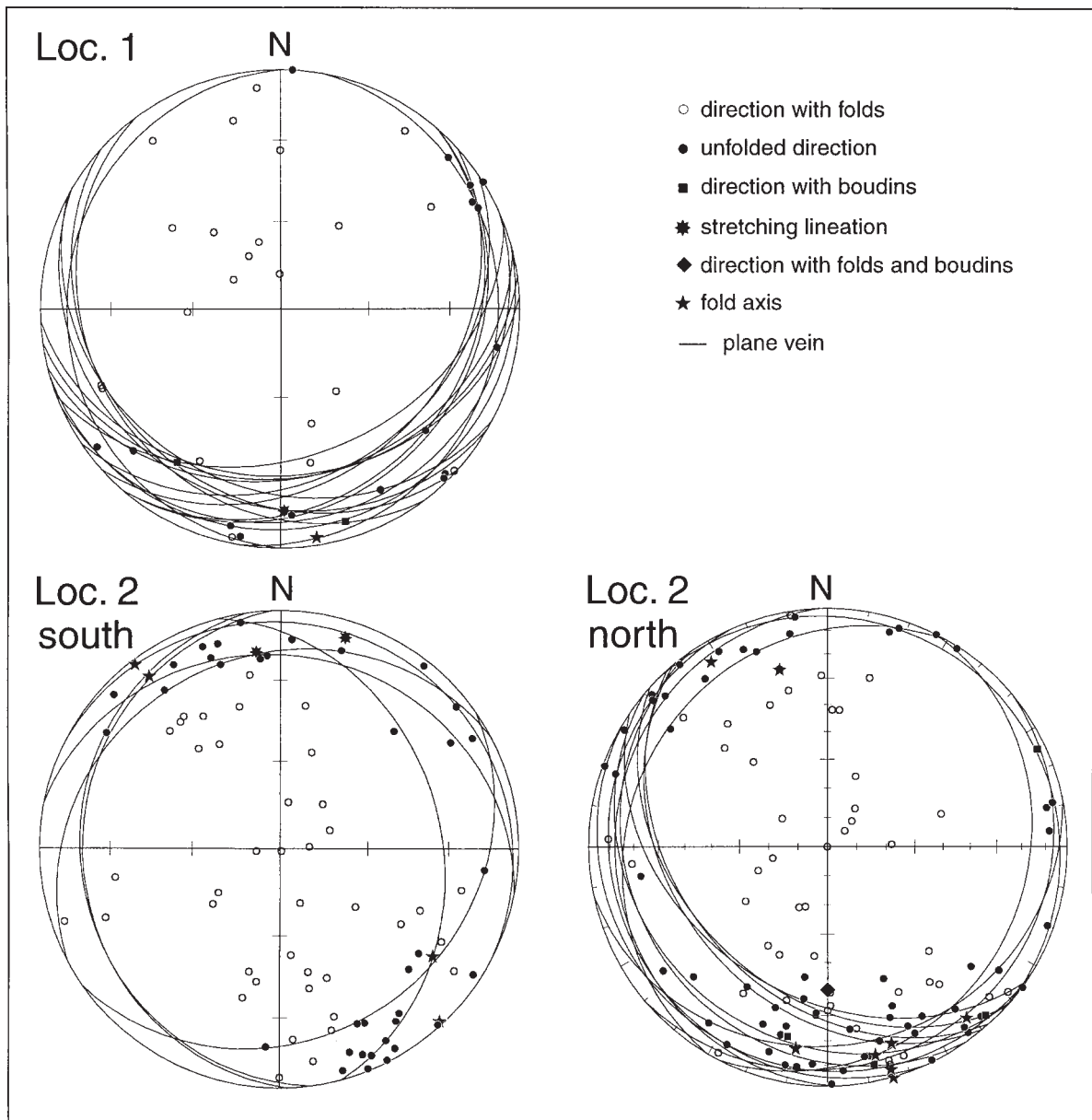
Fig. 10. Plots showing measured orientations of vein traces and unfolded veins (great circles) in the monzonite dykes at locality 1 and 2. Equal area projections, lower hemisphere.
