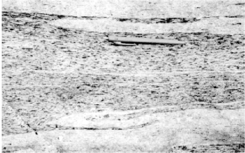
Fig. 6. Above: strongly foliated and lineated monzonite dyke with folded granitic sheets, the lineation is almost parallel to the surface of the outcrop, locality 3, ball pen as scale. Right: thin section showing foliation in a monzonite dyke (plane light), the monzonite also contains a lineation which is perpendicular to the section. Horizontal length of photo is 2 cm.
