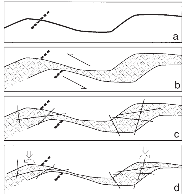
Fig. 13. Simplified cartoon to illustrate the formation of the monzonite dyke at locality 2 (a to b), the emplacement of the granitic veins (c) and a model for the deformation and development of the internal structures (d). The horizontal length of the section is approx. 35 m.
