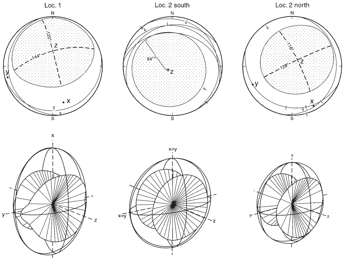
Fig. 11. Above: equal area projections showing shortening fields (stippled) and extension fields; great circles indicate measured foliations and o- indicates a measured fold axis. Below: shapes of the corresponding strain ellipsoids and their surfaces of no finite longitudinal strain, notice that the flattening planes (the XY planes) are vertical in these Figures, while they are subhorizontal at the localities as seen in the stereonet projections above.
