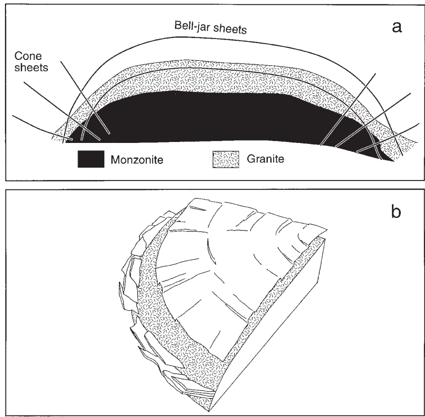
Fig. 3. Simplified profile (a) and block diagram (b) outlining the cone sheets and bell-jar sheets in the Høvringsvatn area.
