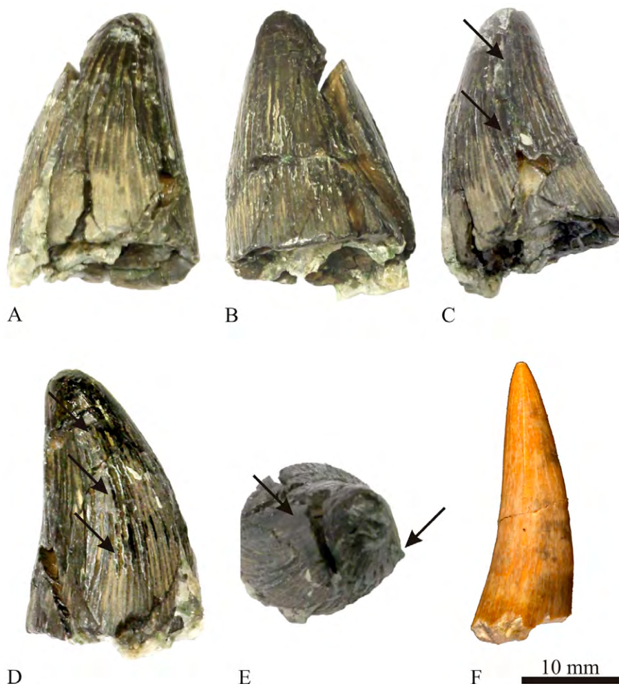
Fig. 3. Isolated crocodylian tooth from the basal conglomerate of the Lelling Greensand Formation (Middle Paleocene) (MGUH-30862), A : Lingual view. B : Labial view. C : Mesial view. D : Distal view. E : In apical aspect. The weak carina (cutting edge) is visible in the mesial, distal and apical views, indicated by arrows. F : Thoracosaurid tooth from the Middle Danian of Faxe Quarry for comparison. Photos A – E by Heinrich Mallison. Photo F by Sten Lennart Jakobsen.
