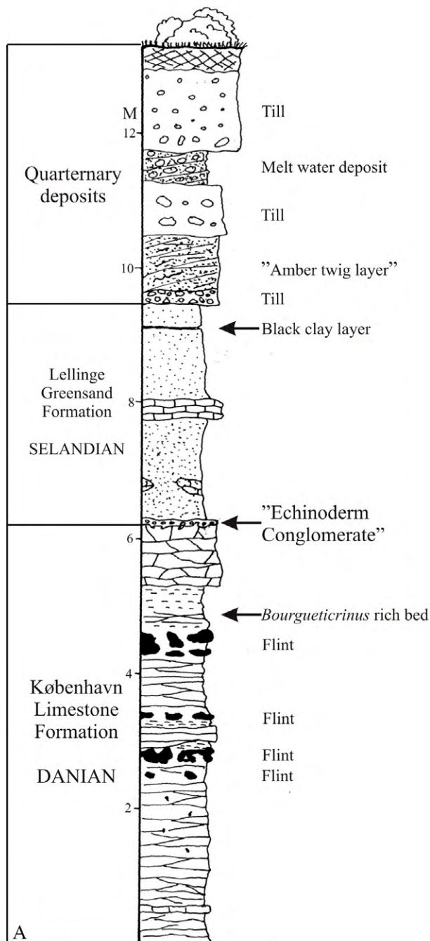
Fig. 2. A: Composite log of the section at the Gemmas Allé site, modified after Gravesen (1994). B: The western part of the excavation near Englandsvej. C: The boundary between the Danian København Limestone Formation and the Selandian Lellinges Greensand Formation. The basal conglomerate of the Lellinges Greensand Formation is indicated by arrow. D: Sample of the conglomerate from the Gemmas Allé site. Note the prominent shark tooth beside the red mark. All photos by Sten Lennart Jakobsen.
