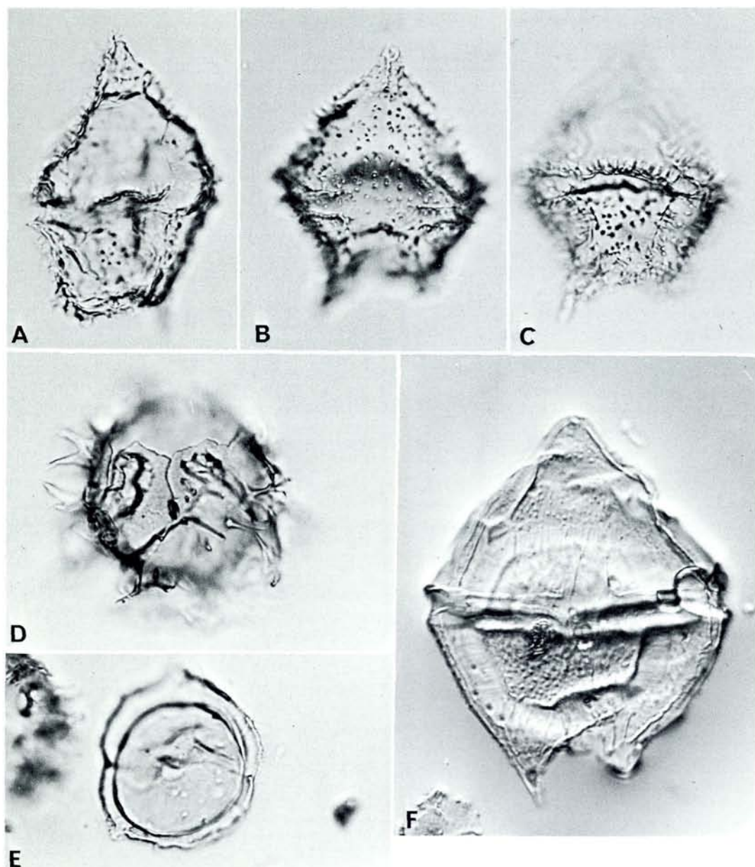
Dinoflagellates from the Bogø boulder. A: Spinidinium densispinatum . B-C: Spinidinium densispinatum , ventral and dorsal sides of the same specimen. D: Areoligera senonensis . E: Paralecaniella indentata . F: Palaeoperidinium pyrophorum . All 750 ×.
