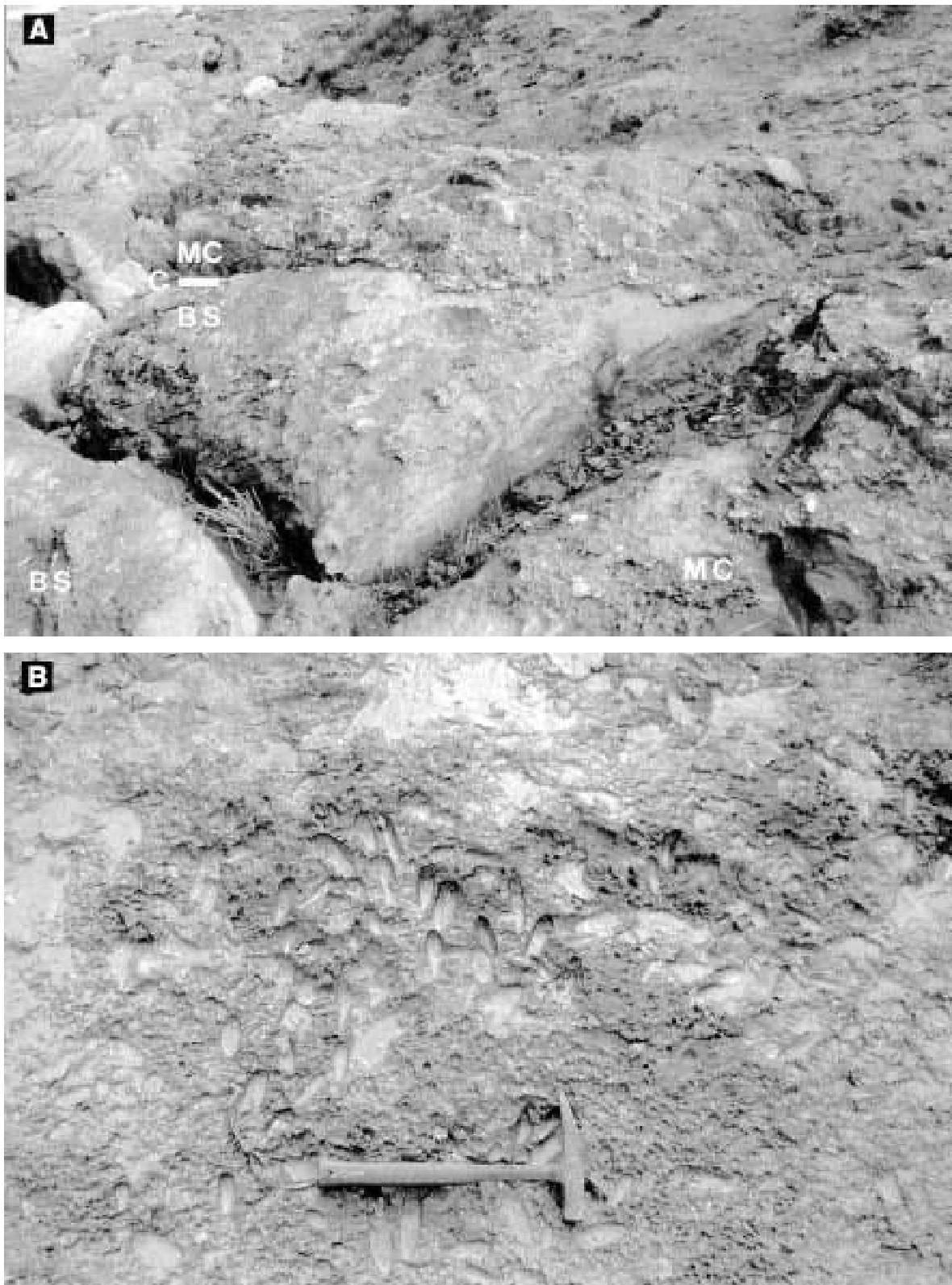
Fig. 2. The Foz da Fonte outcrop (Sesimbra). A, general view of the bioeroded marine-flooding surface and overlying sediments; BS: bioeroded surface (Cretaceous), C: contact, MC: Miocene (Burdigalian) basal conglomerate. B, detail of another sector of the same bioeroded surface. Note the clusters of large, mainly subhorizontal Gastrochaenolites isp. and the smaller, more evenly distributed Gastrochaenolites isp. perpendicular to the bioeroded surface.
