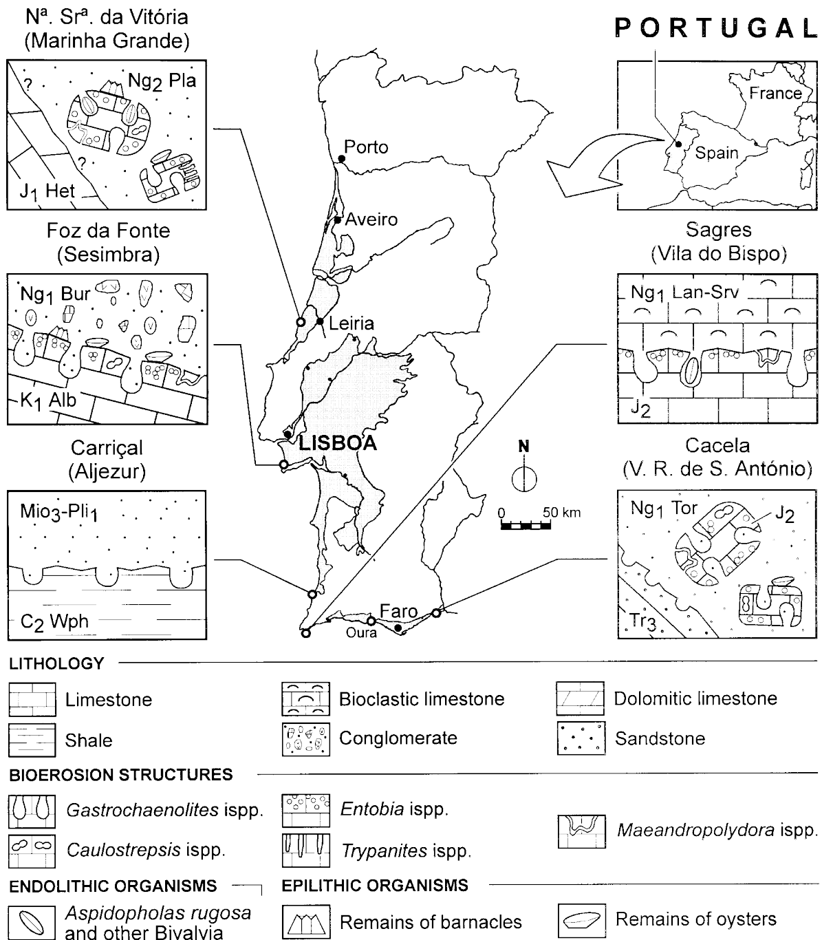
Fig. 1 Geographical location of the Portuguese outcrops featuring Neogene bioerosion structures associated with rocky palaeoshores (modified after Silva et al. 1995). Dotted surface: geographical distribution of the main Neogene outcrops.
